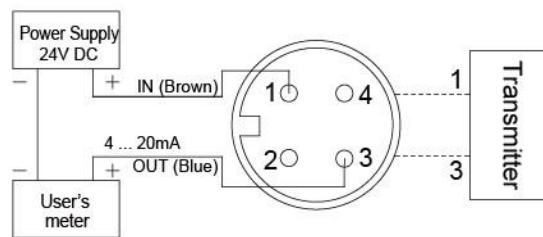
M12 Connector
