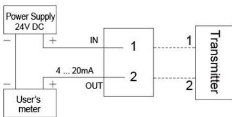
DIN43650 Connector
