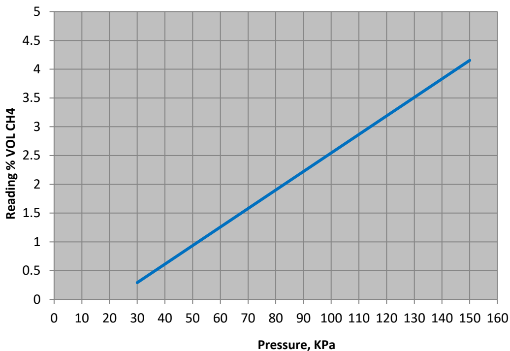
Premier methane sensor pressure dependency, applied gas 2.5% volume methane
